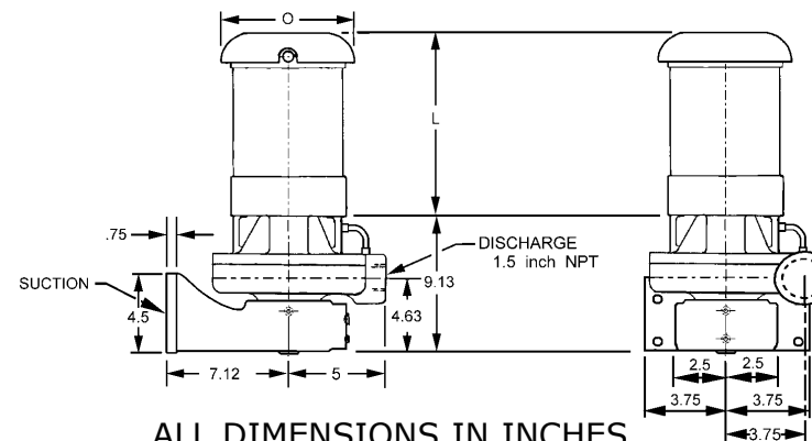
ALL DIMENSIONS IN INCHES
